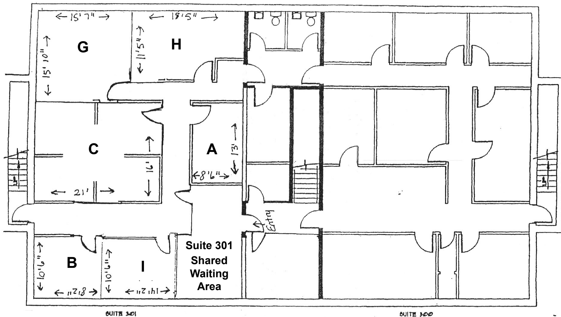
Suite 301 Lower Level Floor Plan
