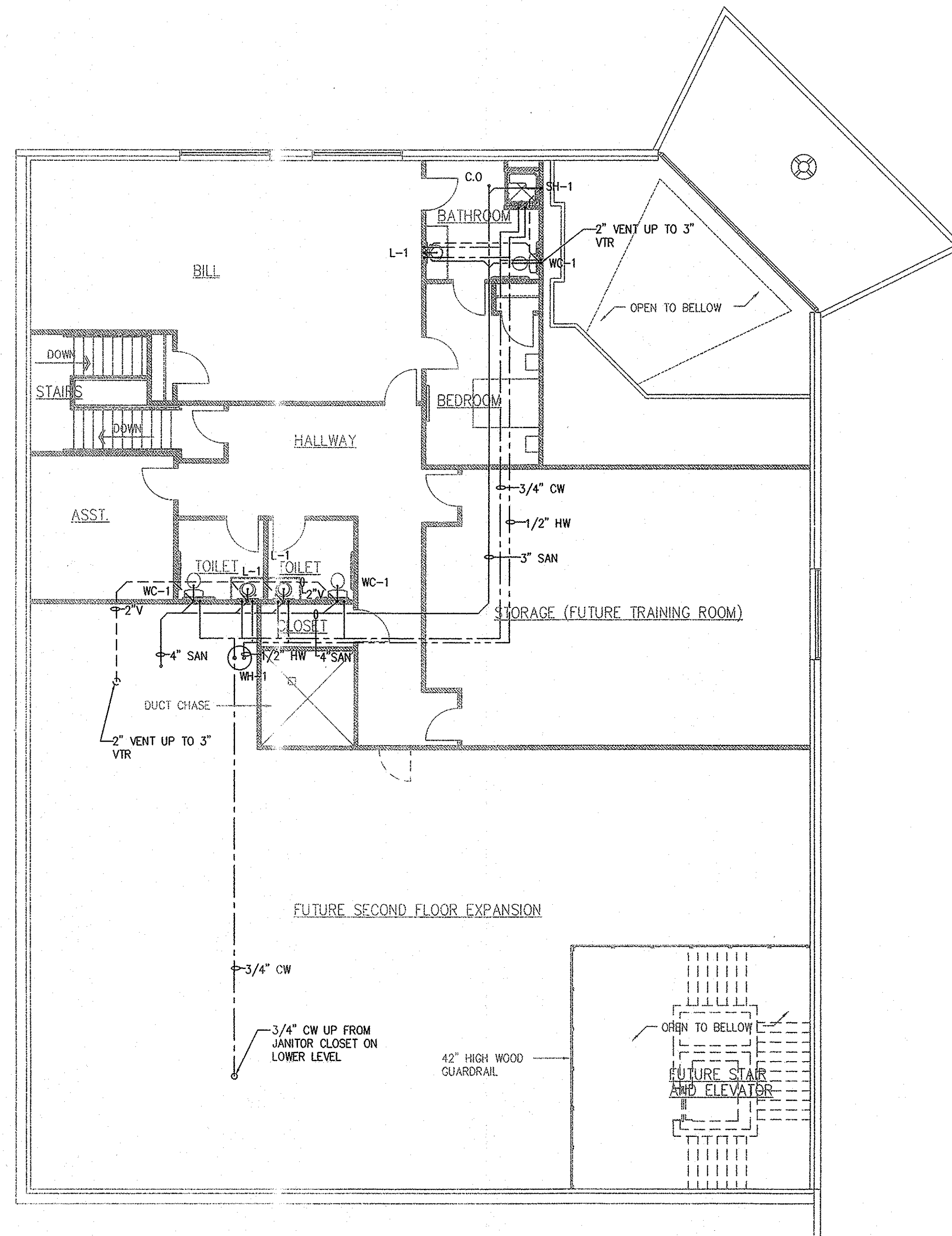
PARTIAL MEZZANINE FLOOR PLAN – INTERIOR FITOUT SCALE: 1/8"=1'-0" MEZZANINE FITOUT AREA: 2,980 SQ. FT.
