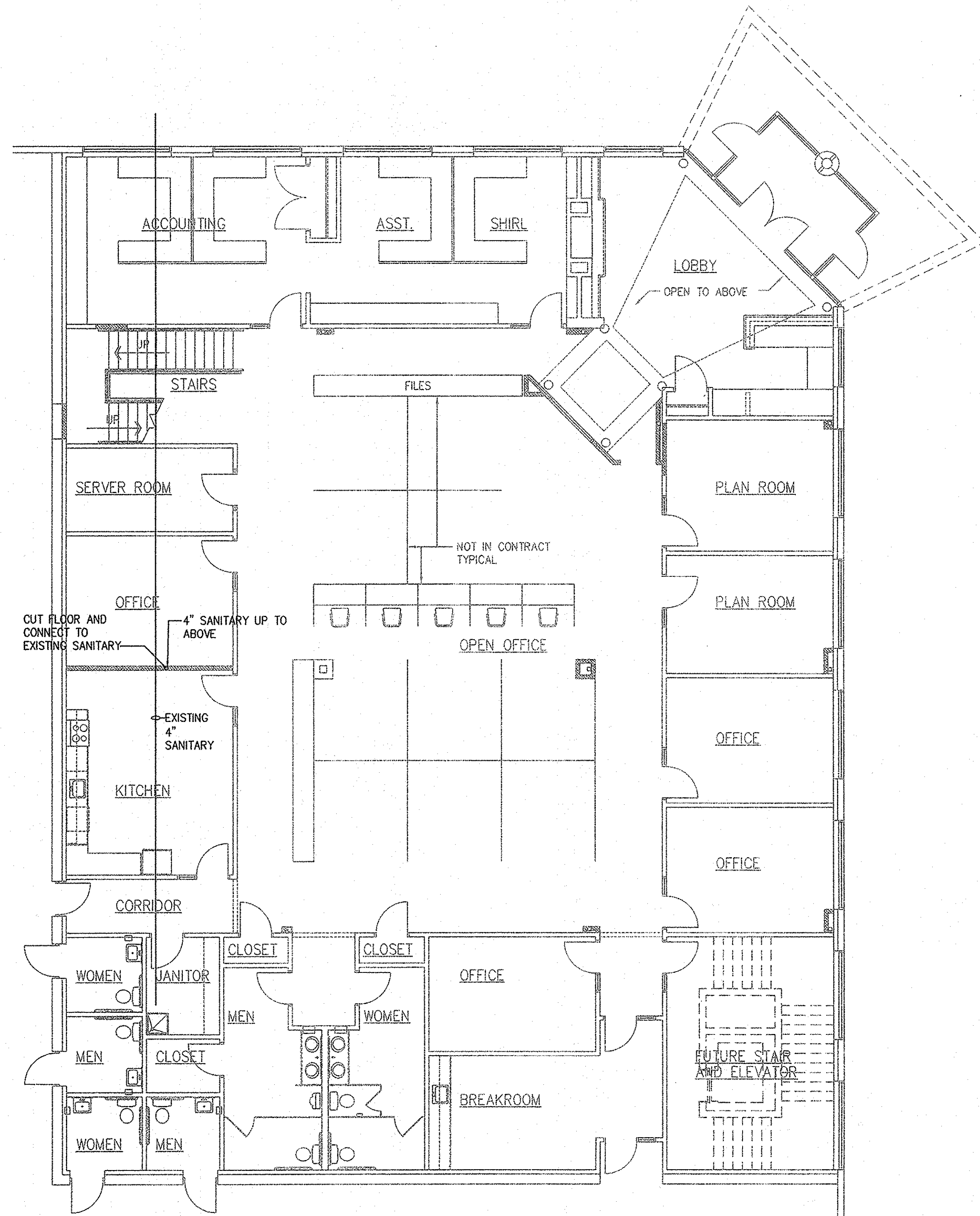
PARTIAL FIRST FLOOR PLAN – INTERIOR FITOUT SCALE: 1/8"=1'-0"
